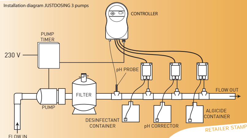
Installation diagram JUSTDOSING 3 pumps
